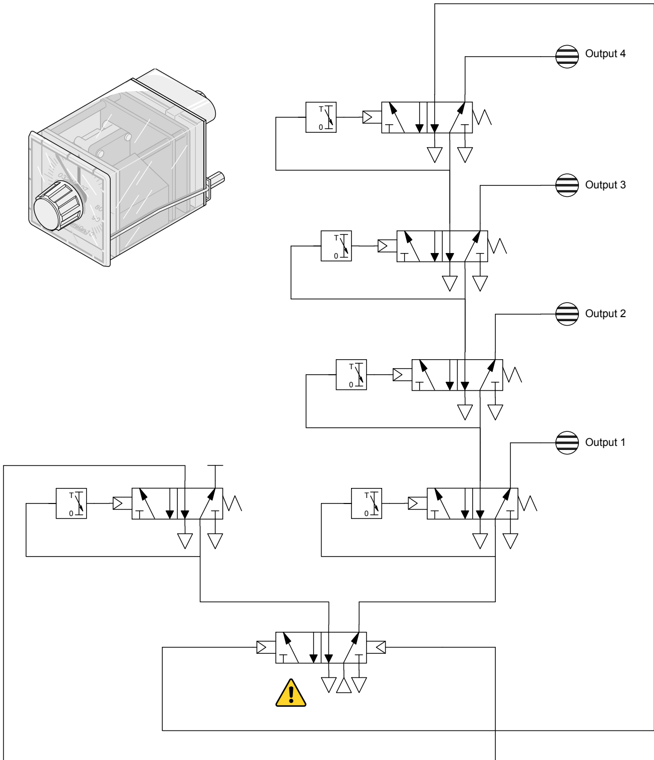
Unattended - 4 x Single shot repeating cascade circuit
