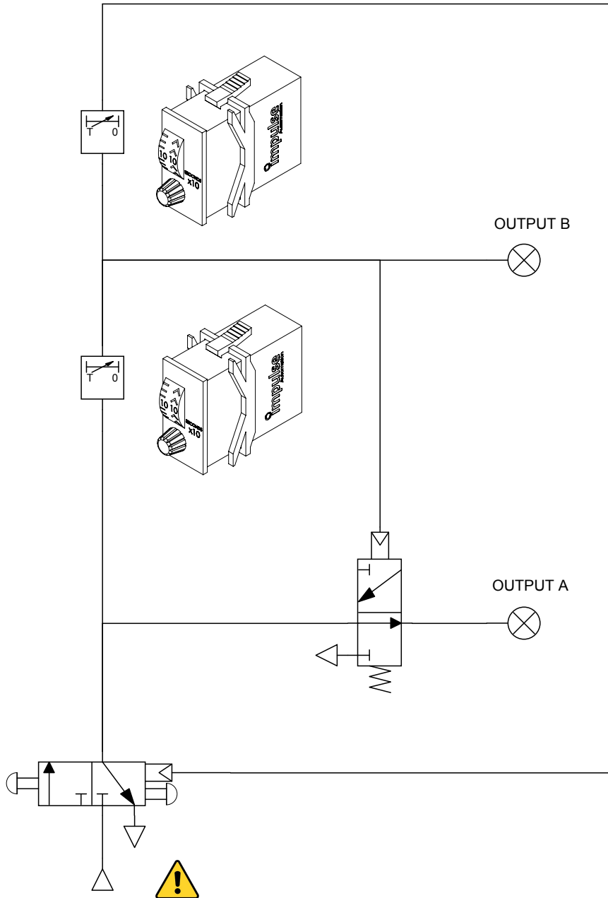
Unattended - Single shot dual timed output circuit with push/pull valve (Start/Stop)
