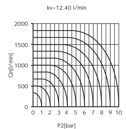
Flow rate orifice spool type
