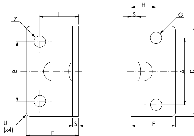
Mounting brackets Piston Ø 40 - 100 mm 2 pieces provided Inc. fixing bolts
