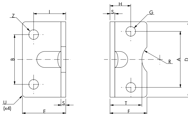
Mounting brackets Piston Ø 12 - 32 mm 2 pieces provided Inc. fixing bolts
