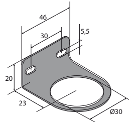
Mounting Bracket (G3/8 & G1/2)
