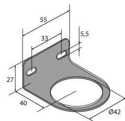
Mounting Bracket (G3/8)
